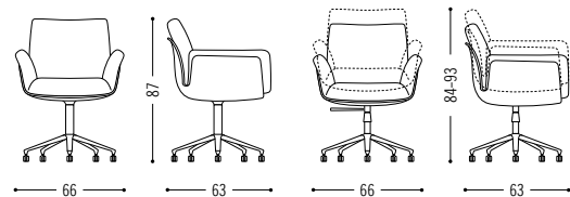
swivel chair 5-star base on castors
