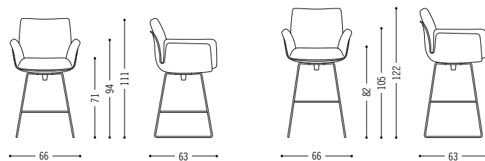
swivel frame
