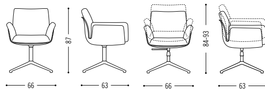
swivel chair 4-star base
