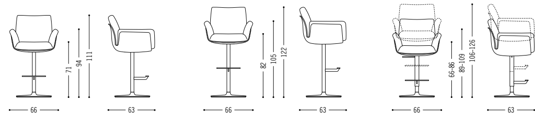
plate base
