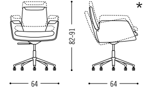
swivel chair 5-star base on castors
